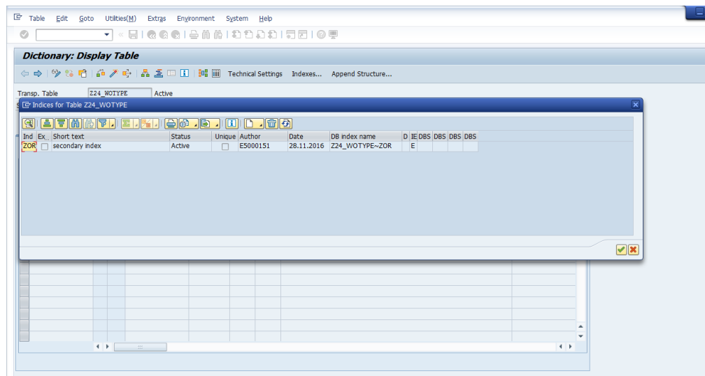
Figure 11-5 Activate Index
