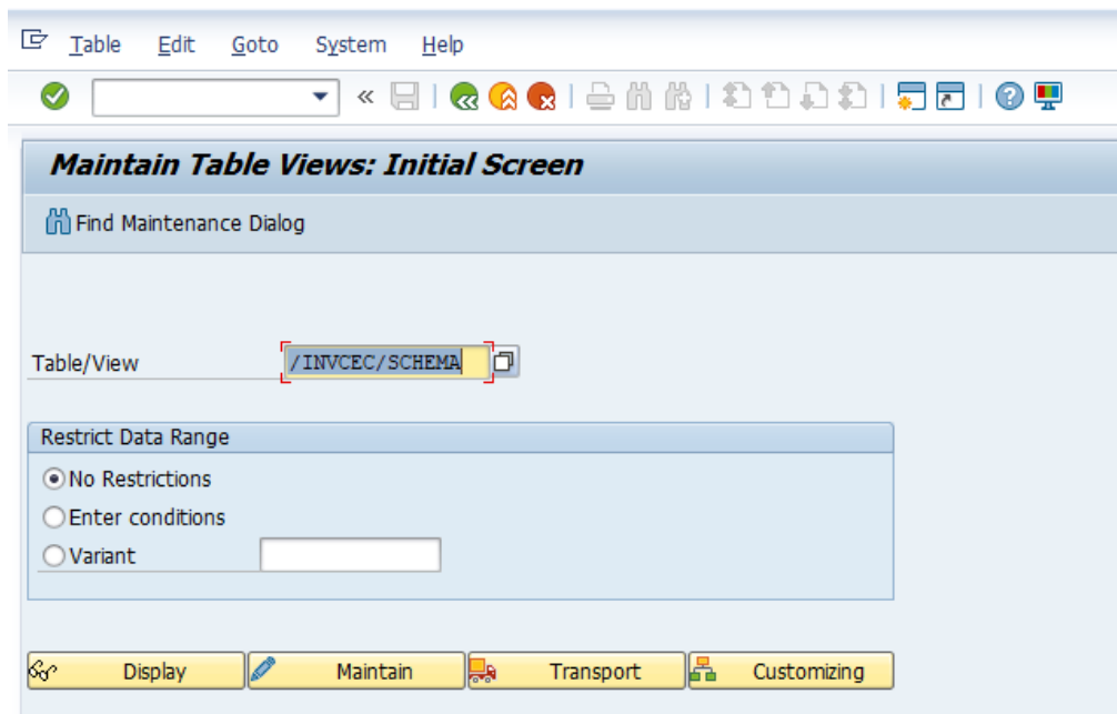
Figure 4-1 SM30
