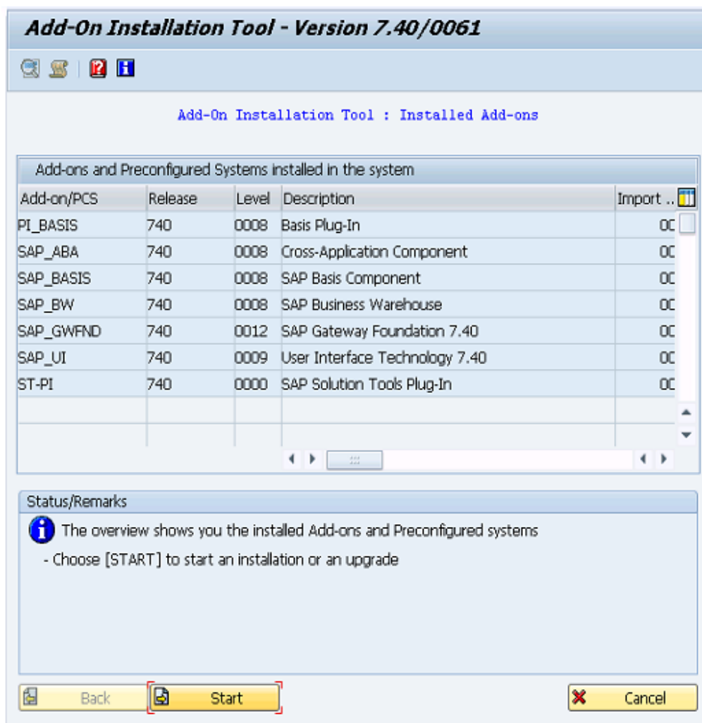
Figure 3-3 Installed Add-ons
