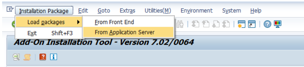
Figure 3-1 SAINT
