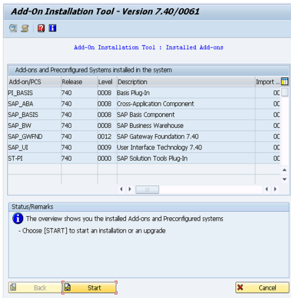
Figure 2-3 Installed Add-ons
