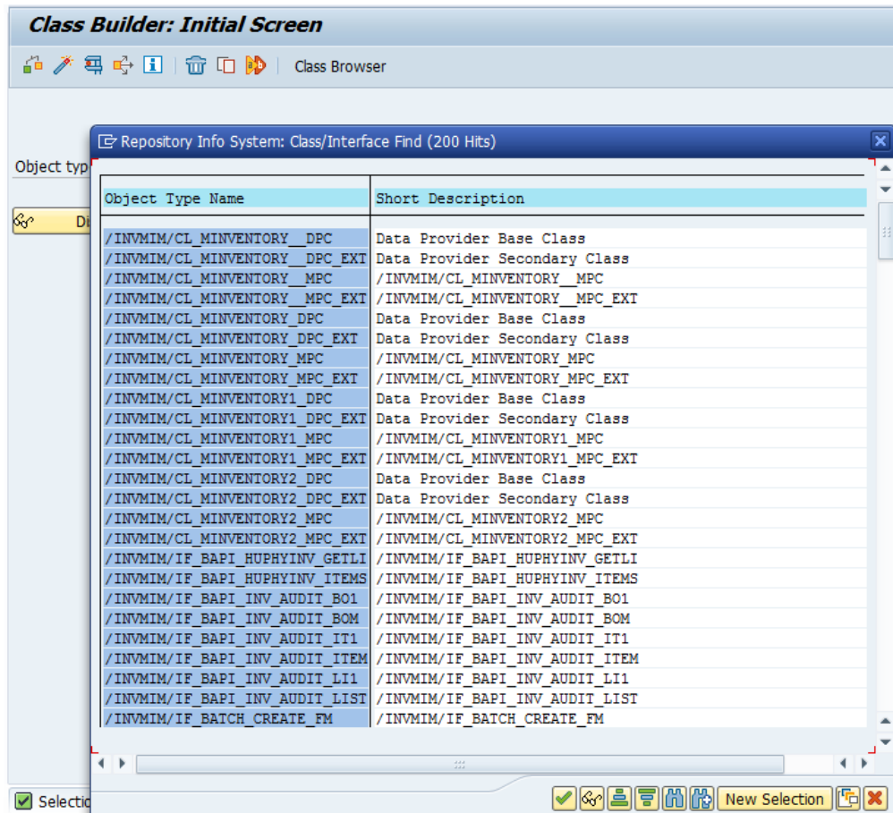
Figure 3-9 Object Classes
