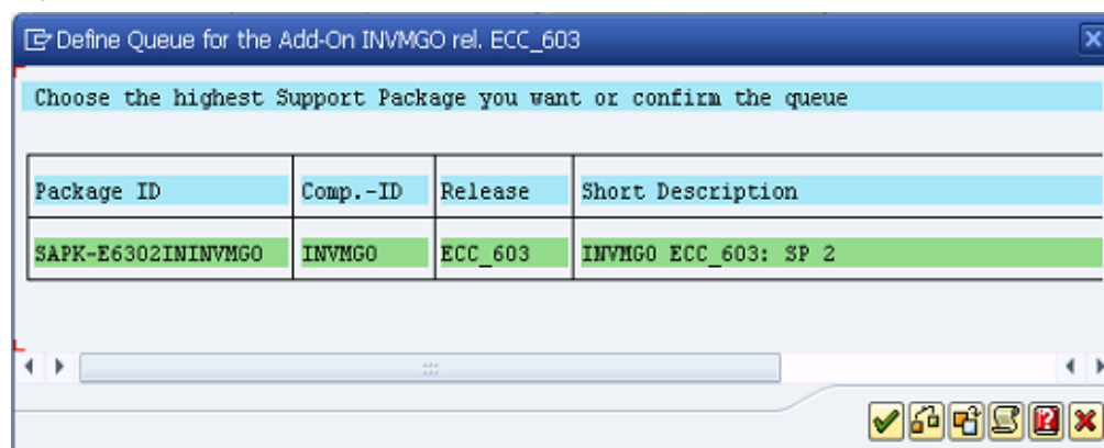
Figure 3-14 Confirm Queue
