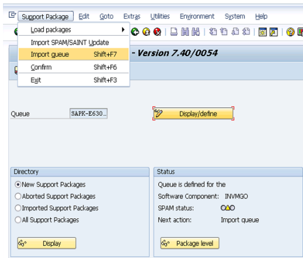
Figure 2-14 Import Queue
