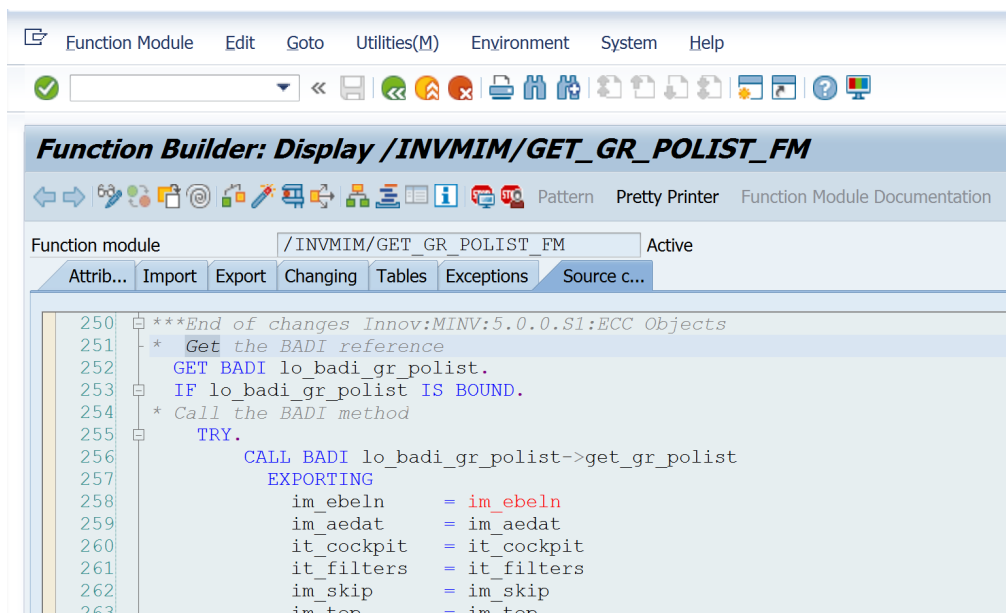
Figure 10–3 FM: /INVMIM/GET_GR_POLIST_FM
