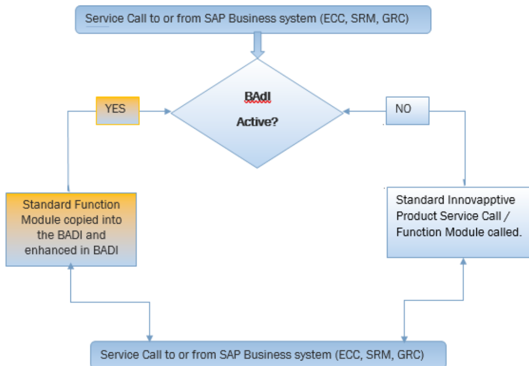
Figure 10-1 BADI Implementation
