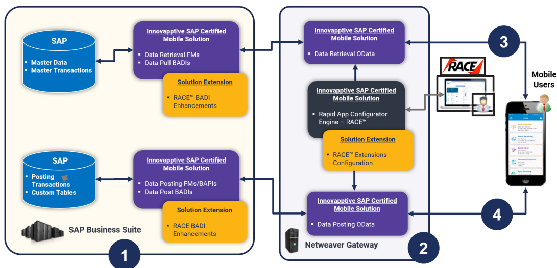
Figure 7-1 RACE™ Architecture
