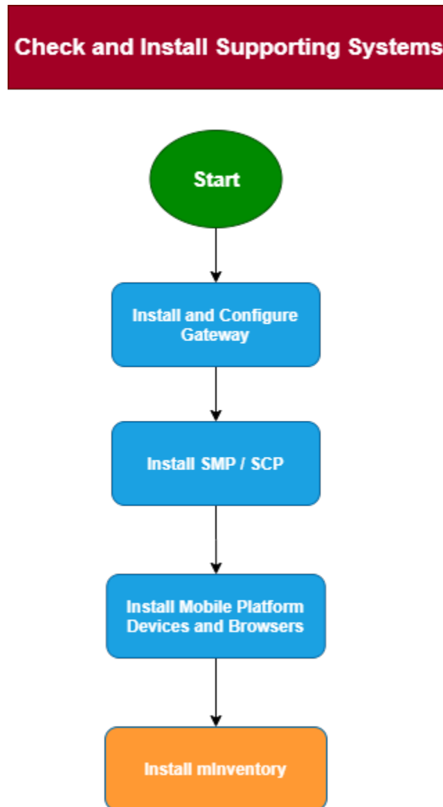
Figure 1-1 Install Systems
