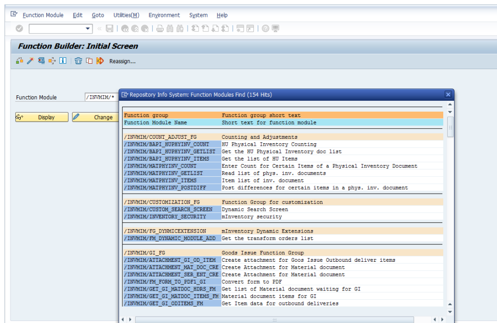
Figure 3-7 Function Modules
