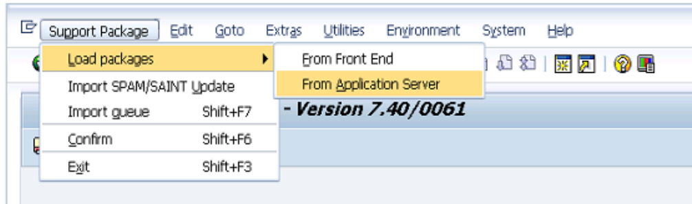
Figure 3-10 SAINT
