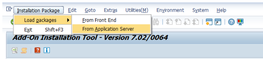
Figure 2-1 SAINT
