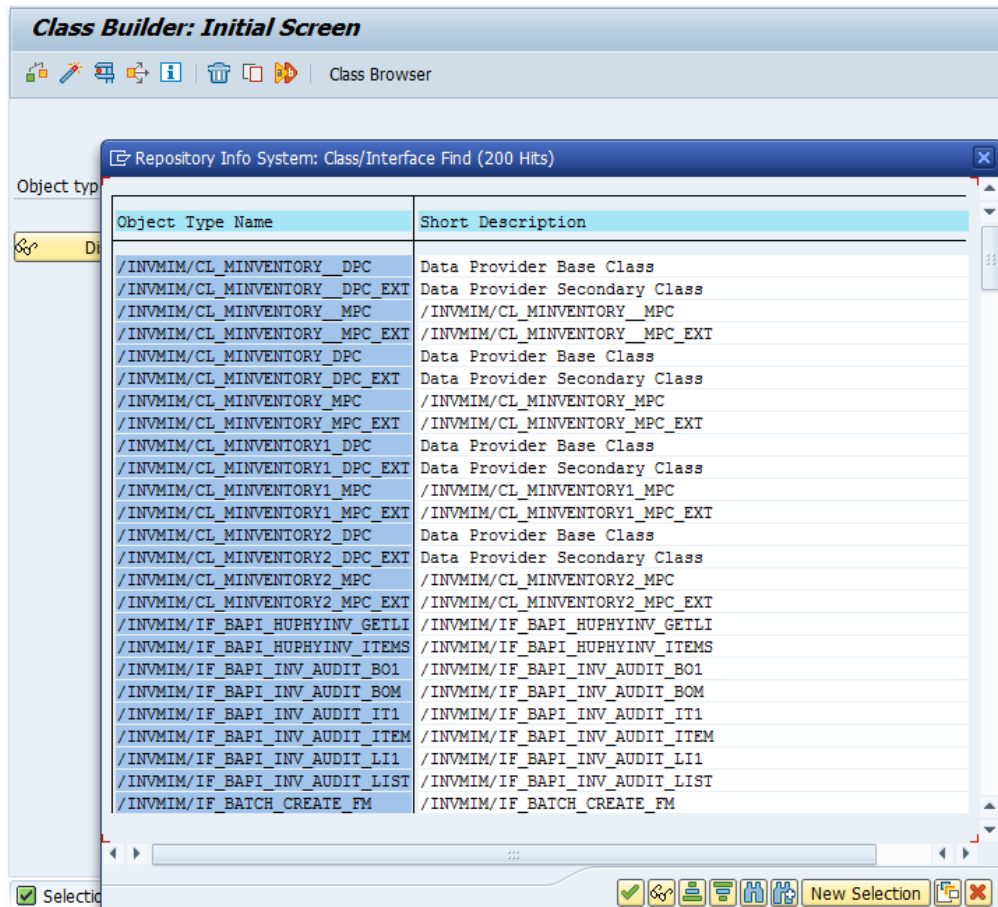
Figure 3-23 Object Classes
