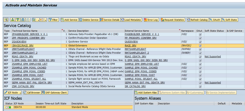
Figure 3–34 Service Status
