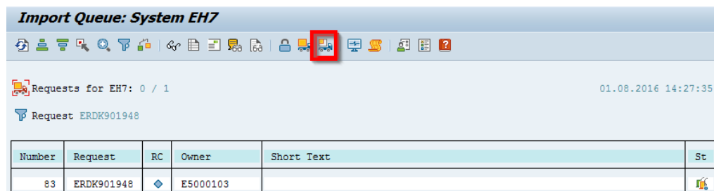
Figure 3-27 Import Queue
