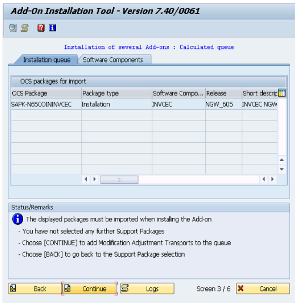
Figure 4-5 Add-on Queue
