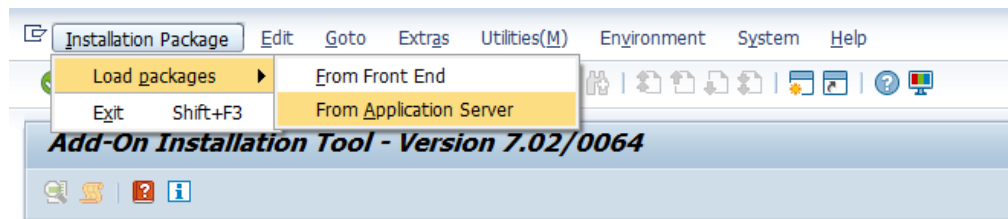
Figure 4-1 SAINT
