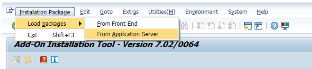
Figure 3-1 SAINT
