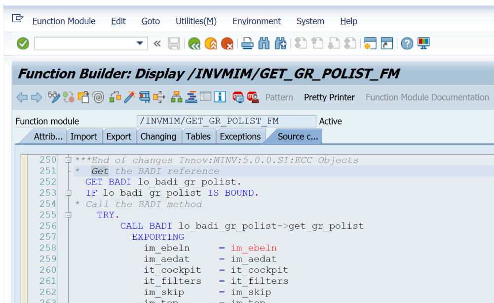
Figure 11-3 FM: /INVMIM/GET_GR_POLIST_FM
