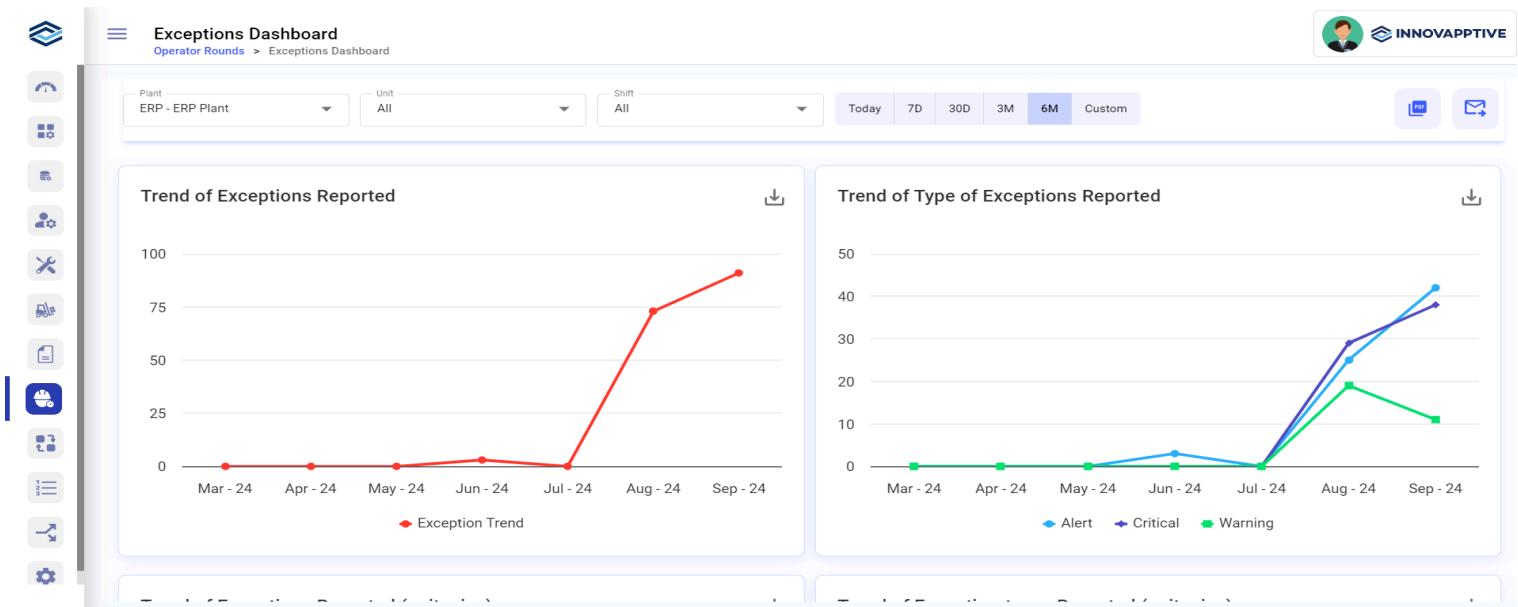
Figure 3-22 Exceptions Dashboard
