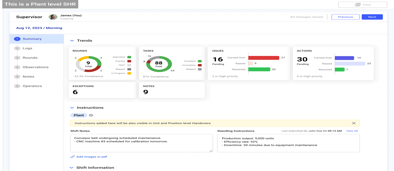
Figure 3-73 SHR Summary
