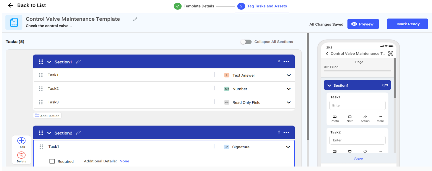
Figure 3-64 Template Preview
