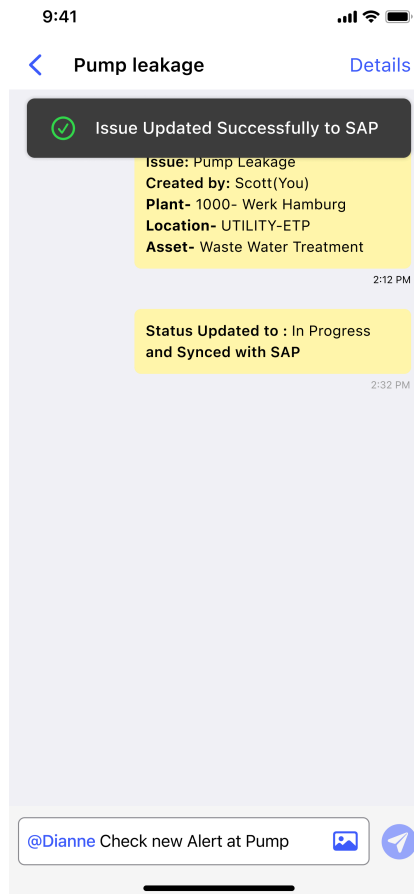
Figure 3-69 SAP Notification
