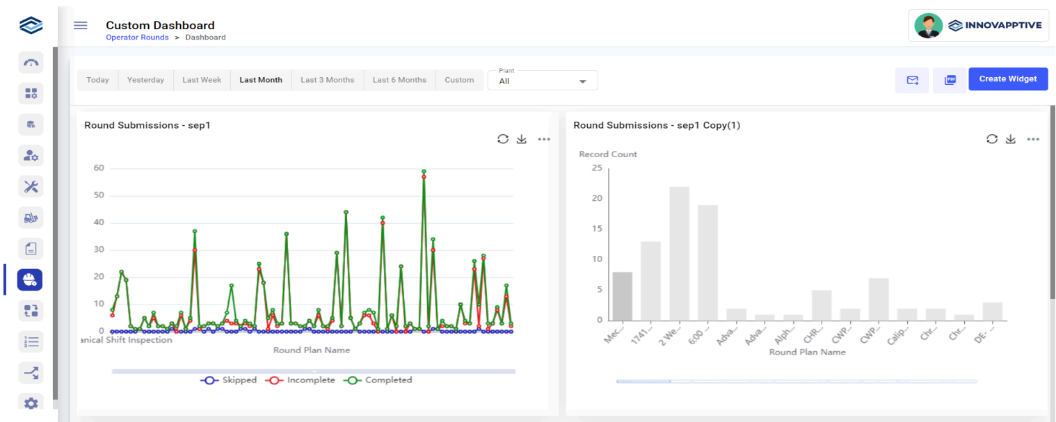
Figure 3-15 Custom Dashboard
