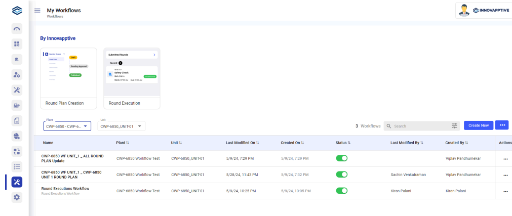
Figure 3-53 My Workflows
