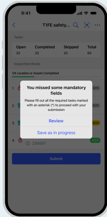
Figure 2-30 Submit Round
