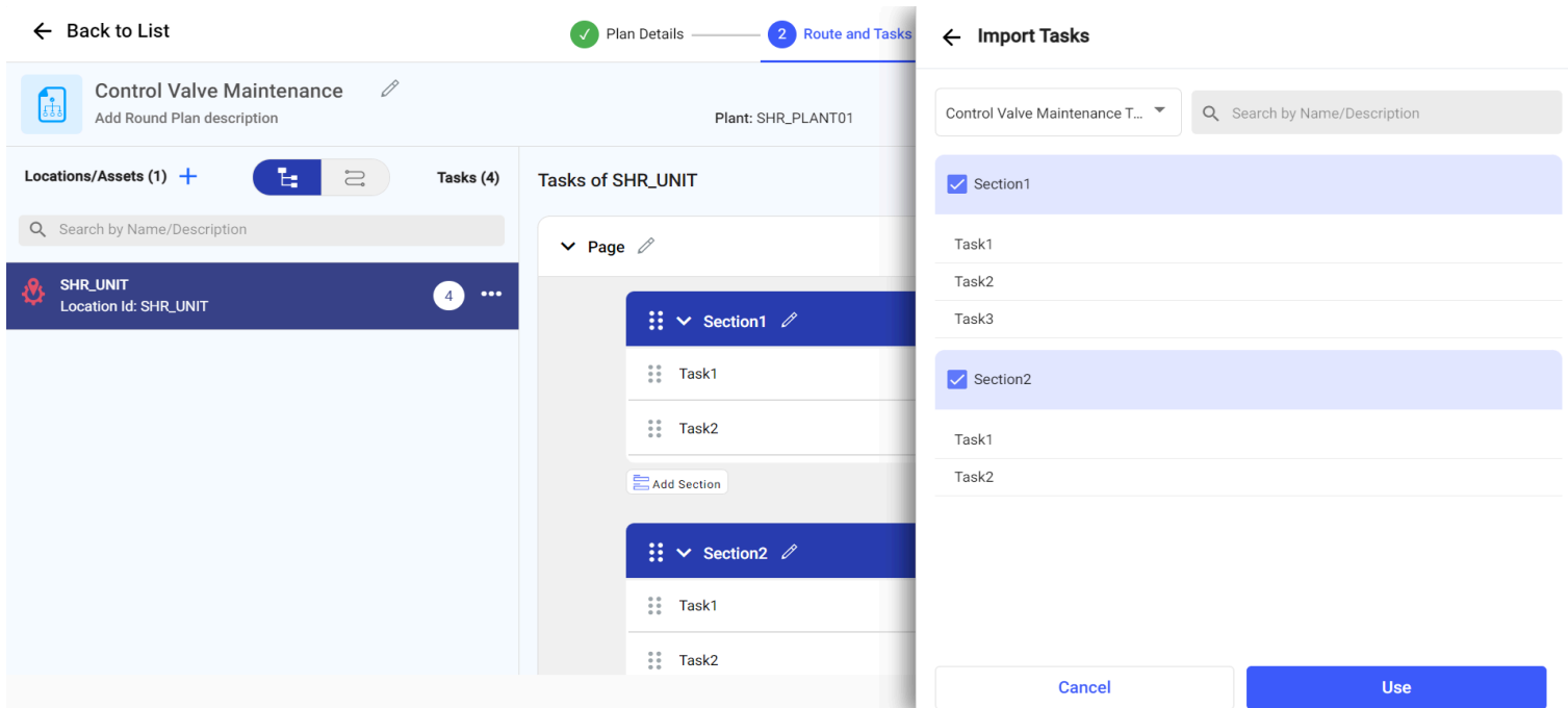
Figure 3-47 Import Tasks
