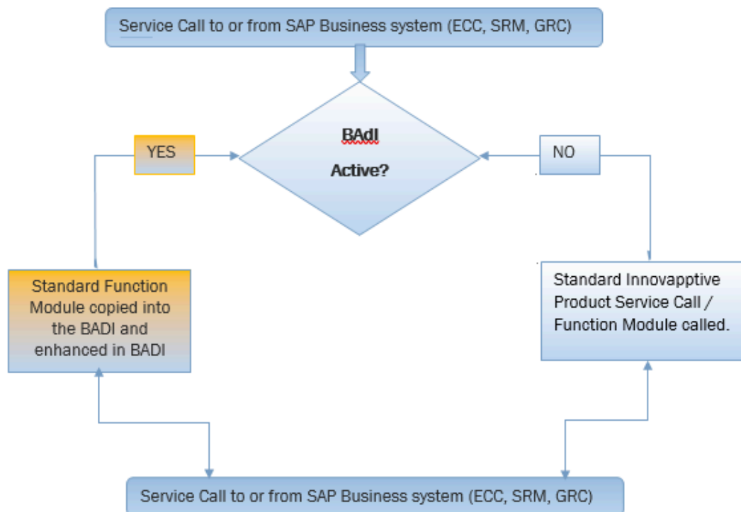
Figure 12-1 BADI Implementation
