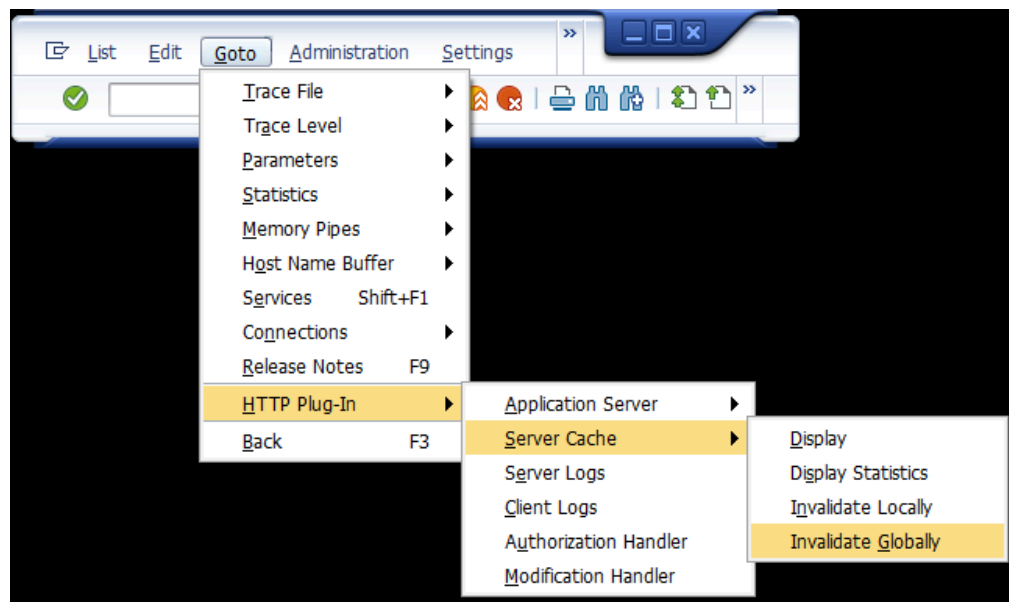
Figure 4-1 smicm transaction
