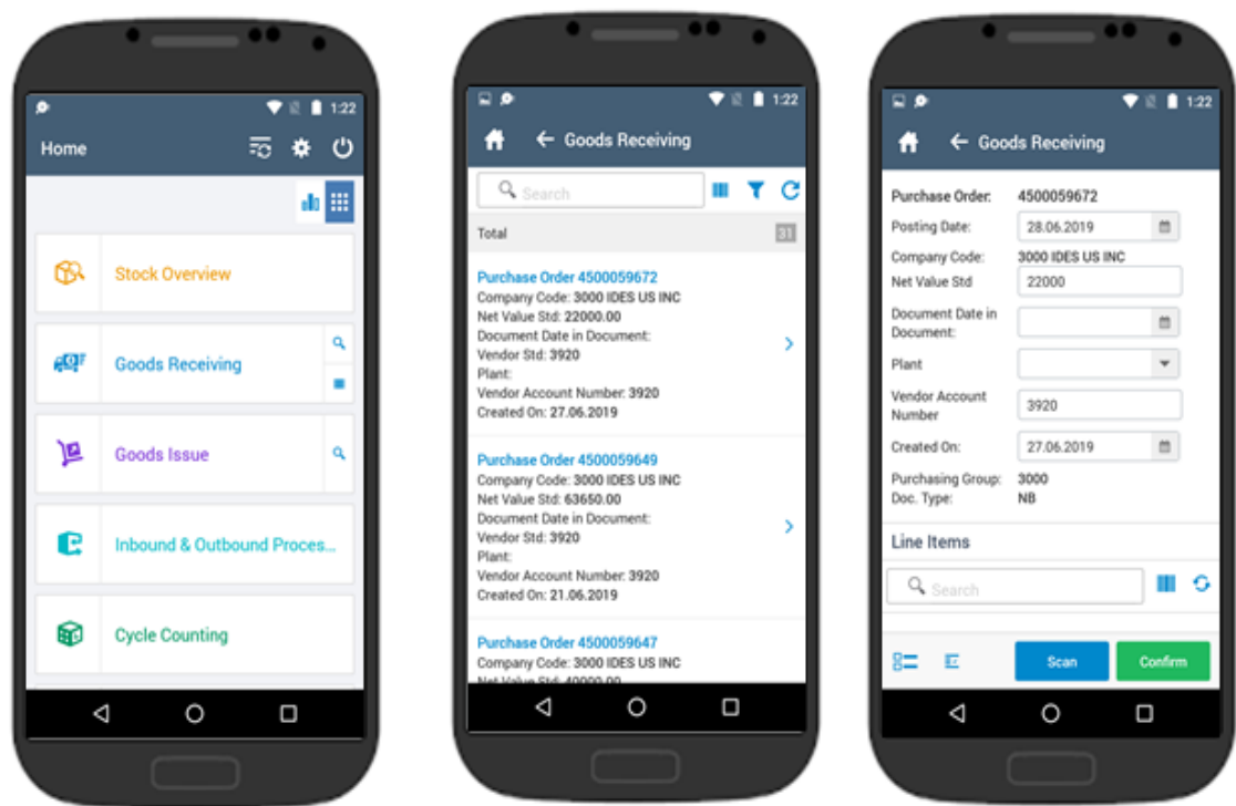
Figure 26-4 Android Screen
