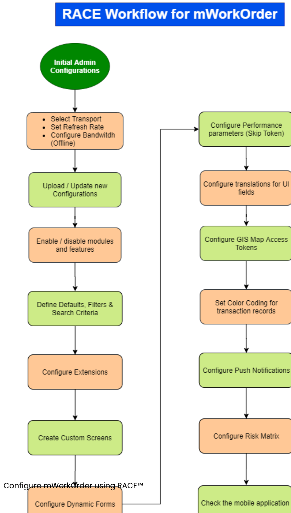
Figure 1-2 RACE Workflow
