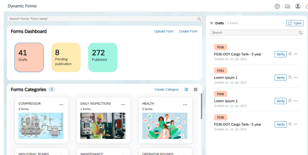
Figure 8-4 Drafted Forms
