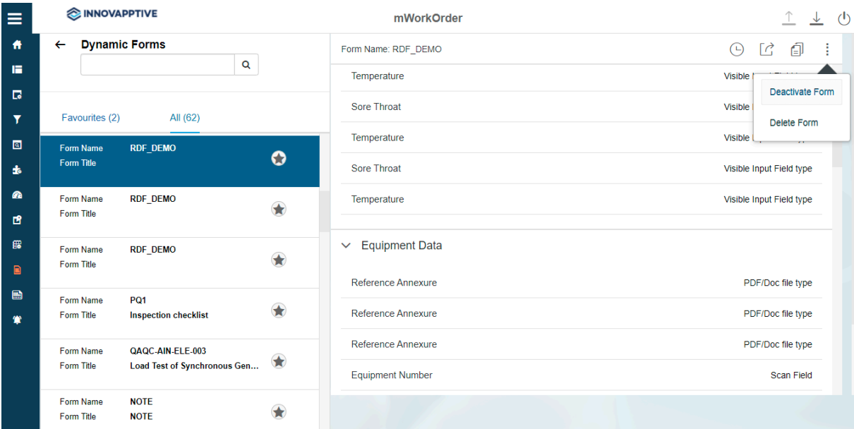
Figure 8–10 Deactivate Form
